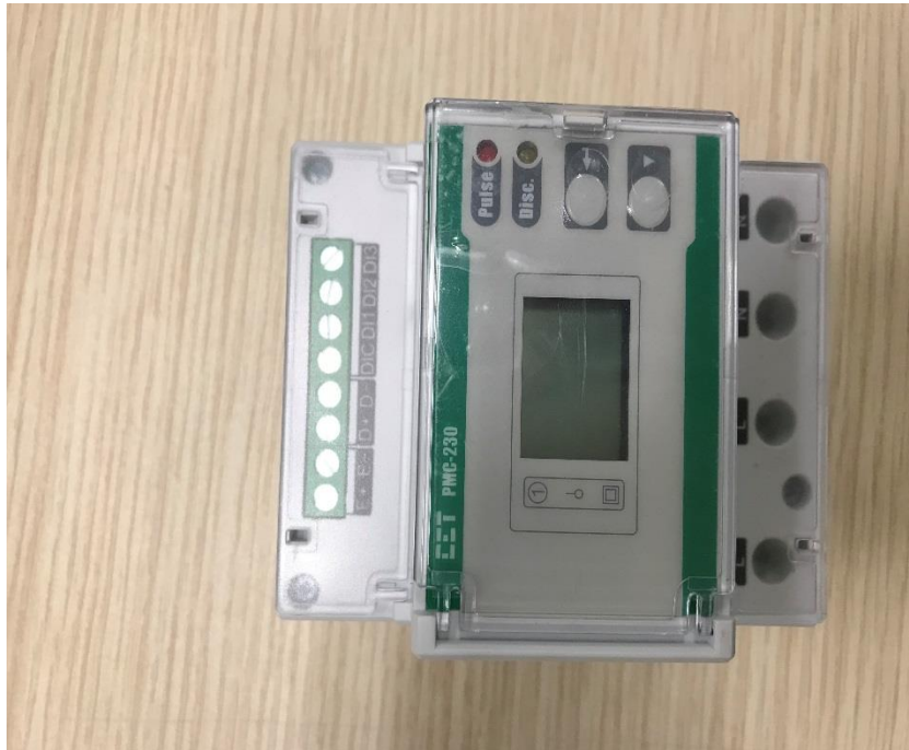
CET Electric Technology Inc. model CET PMC-230-BC35AE Electricity Meter (The Pattern)
